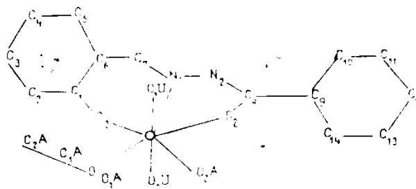
Fig. 2. General view of the molecule.
