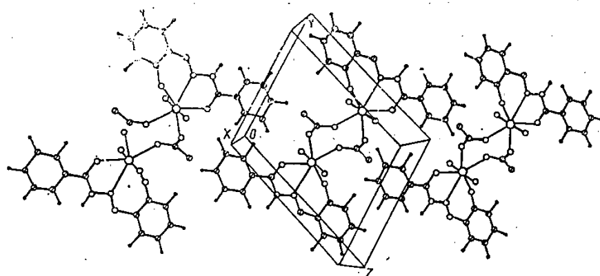
Fig. 1. Packing of complex U(VI) molecules in the structure.
